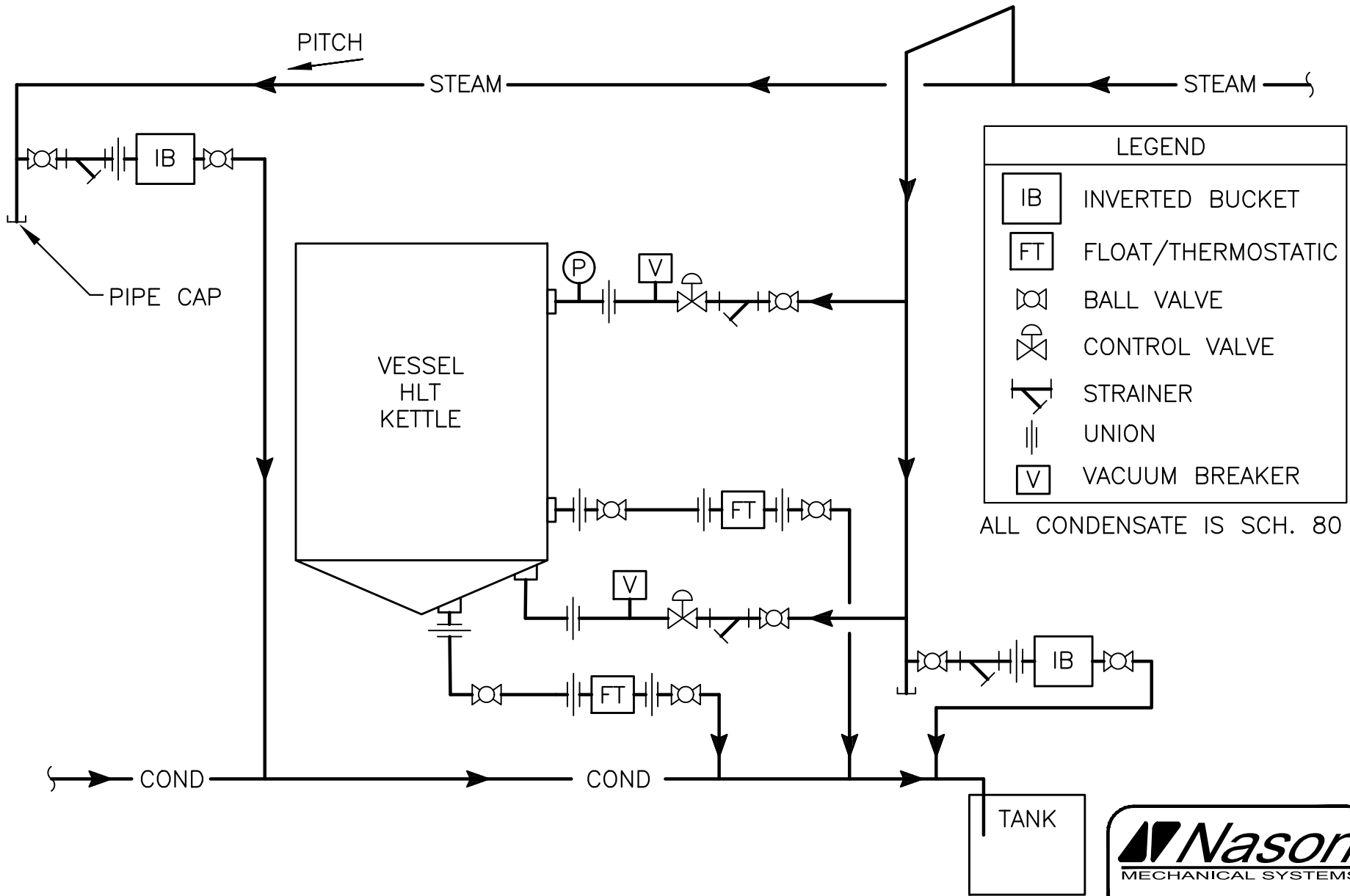
BREWERY EQUIPMENT – TYPICAL STEAM VESSEL PIPING DIAGRAM N.T.S.
