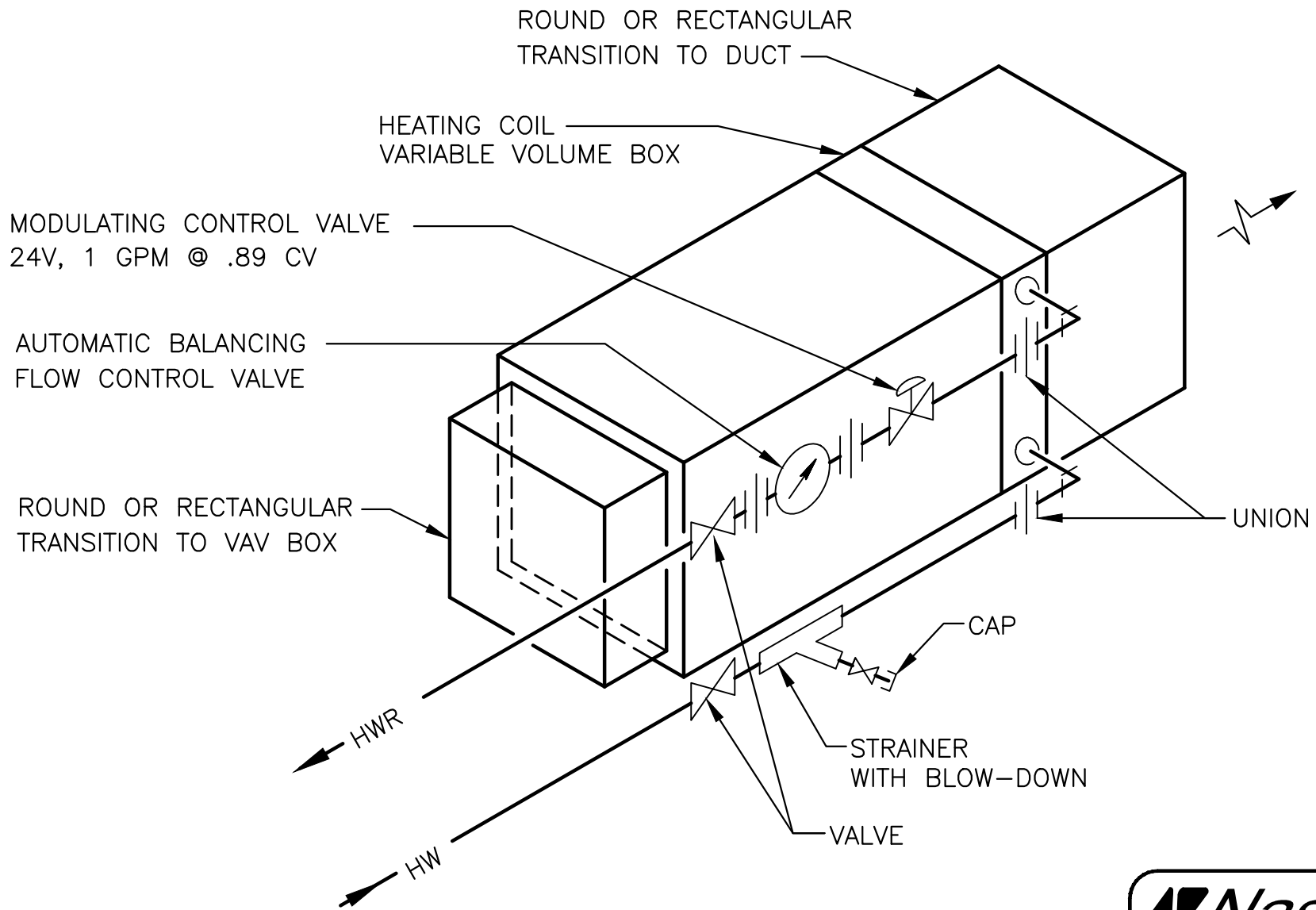
VARIABLE VOLUME BOX WITH REHEAT COIL DETAIL N.T.S.
