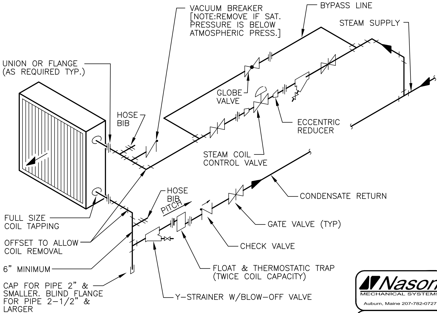
STEAM COIL PIPING DETAIL
