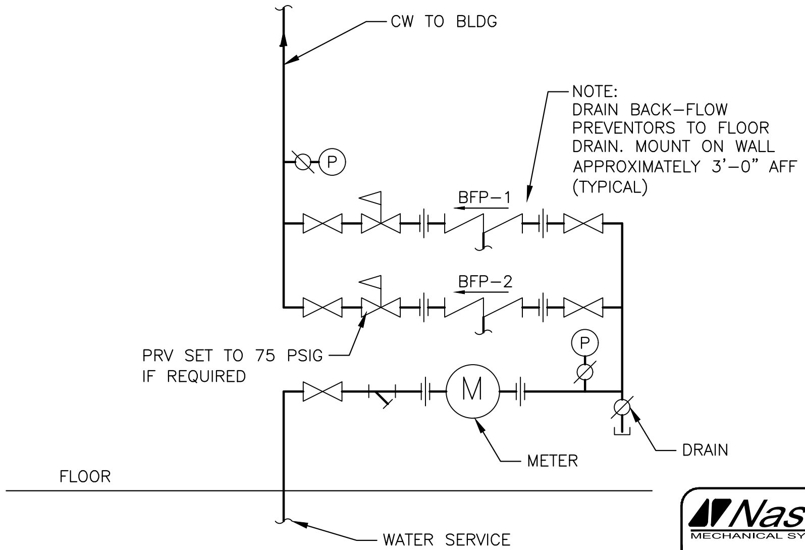
WATER ENTRANCE DETAIL N.T.S.
