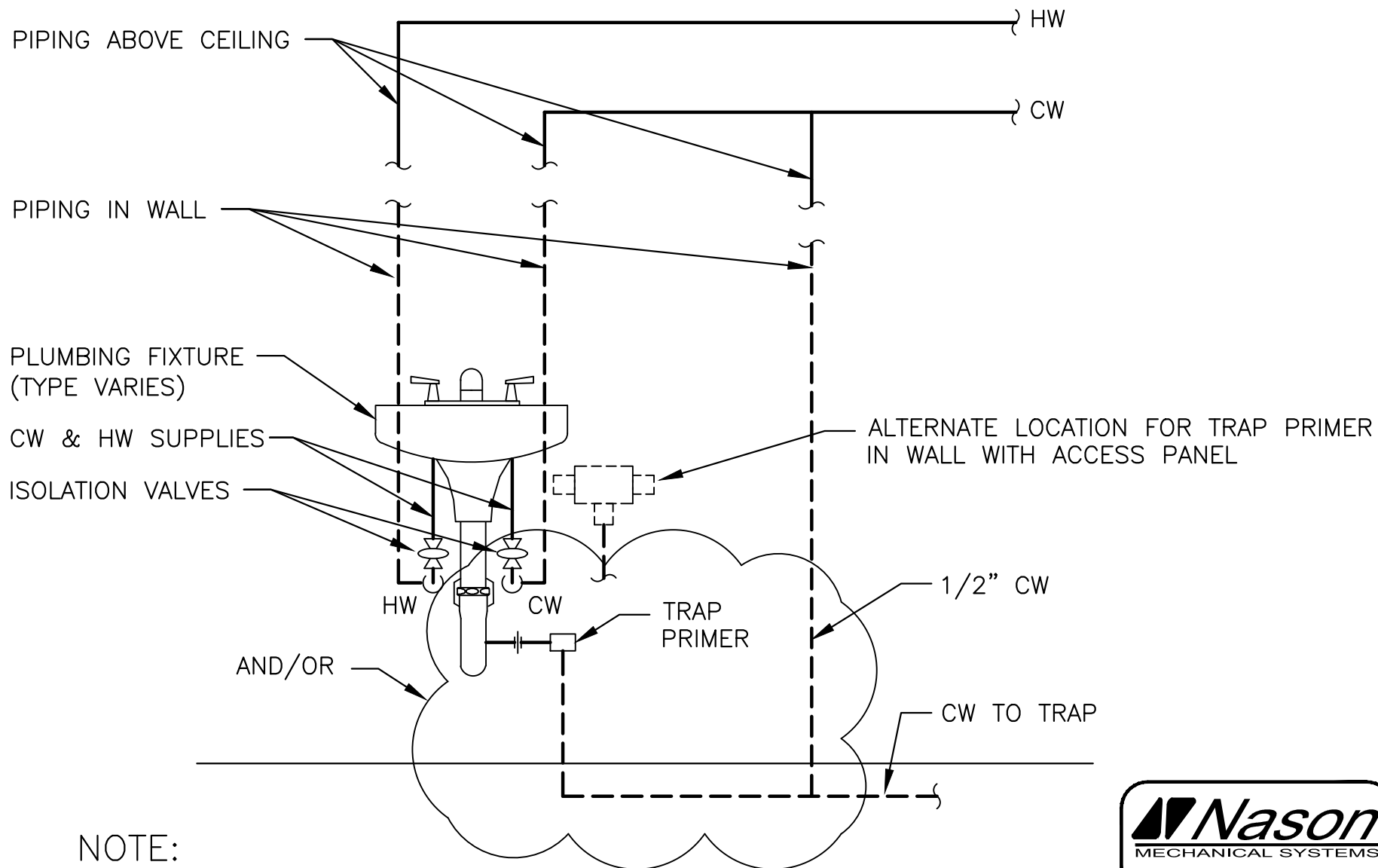
TRAP PRIMER CONNECTION AT SINK DETAIL
